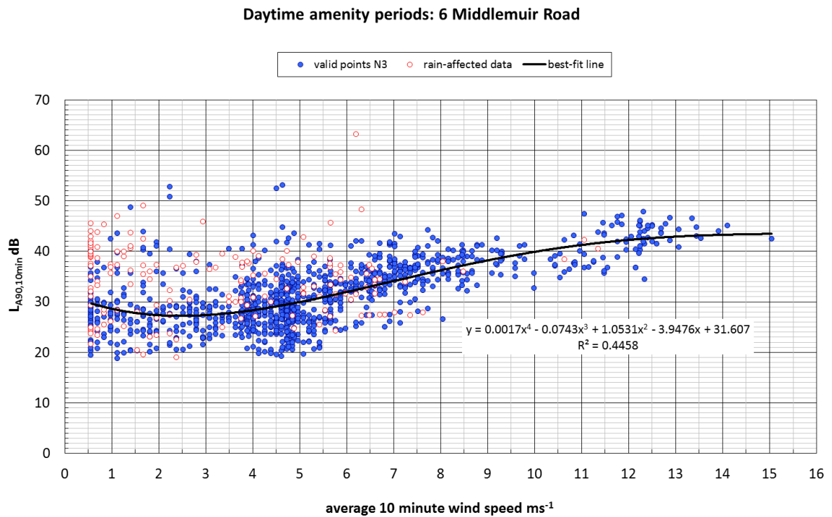
Figure 1 – Background Noise against Wind Speed at 6 Middlemuir Road
