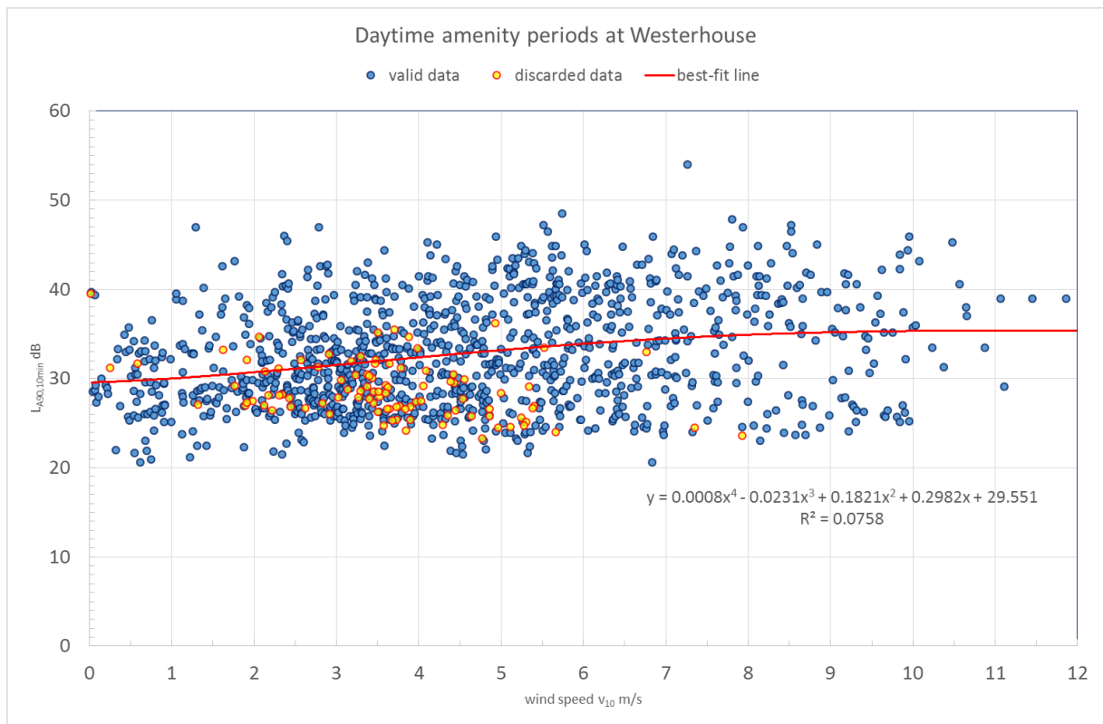
Figure 1 – Background Noise against Wind Speed at Westerhouse
