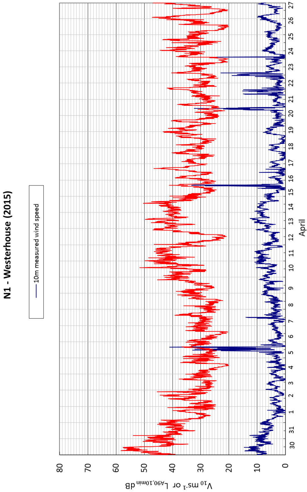
Figure 4 – Time History at Westerhouse (2015)
