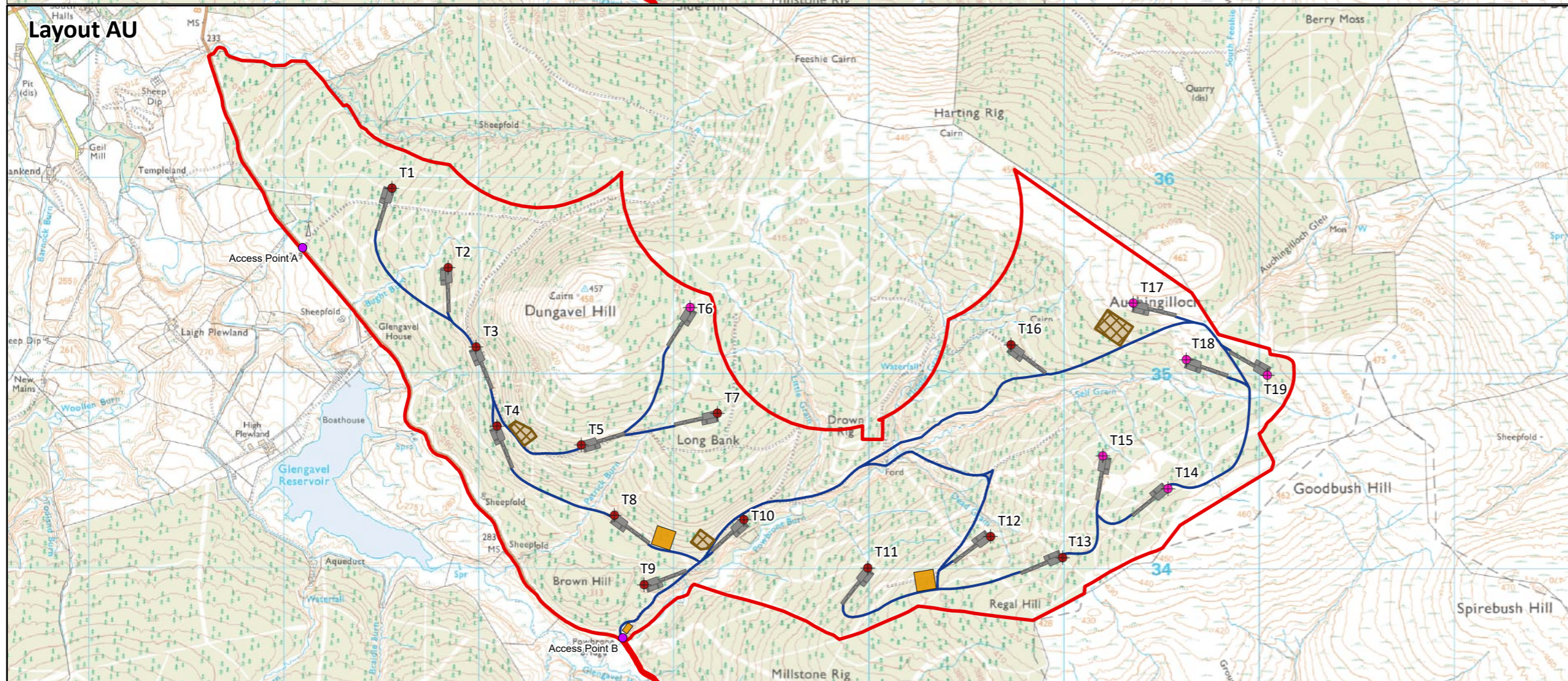
Figure 2.6 Layout AS and Layout AU
