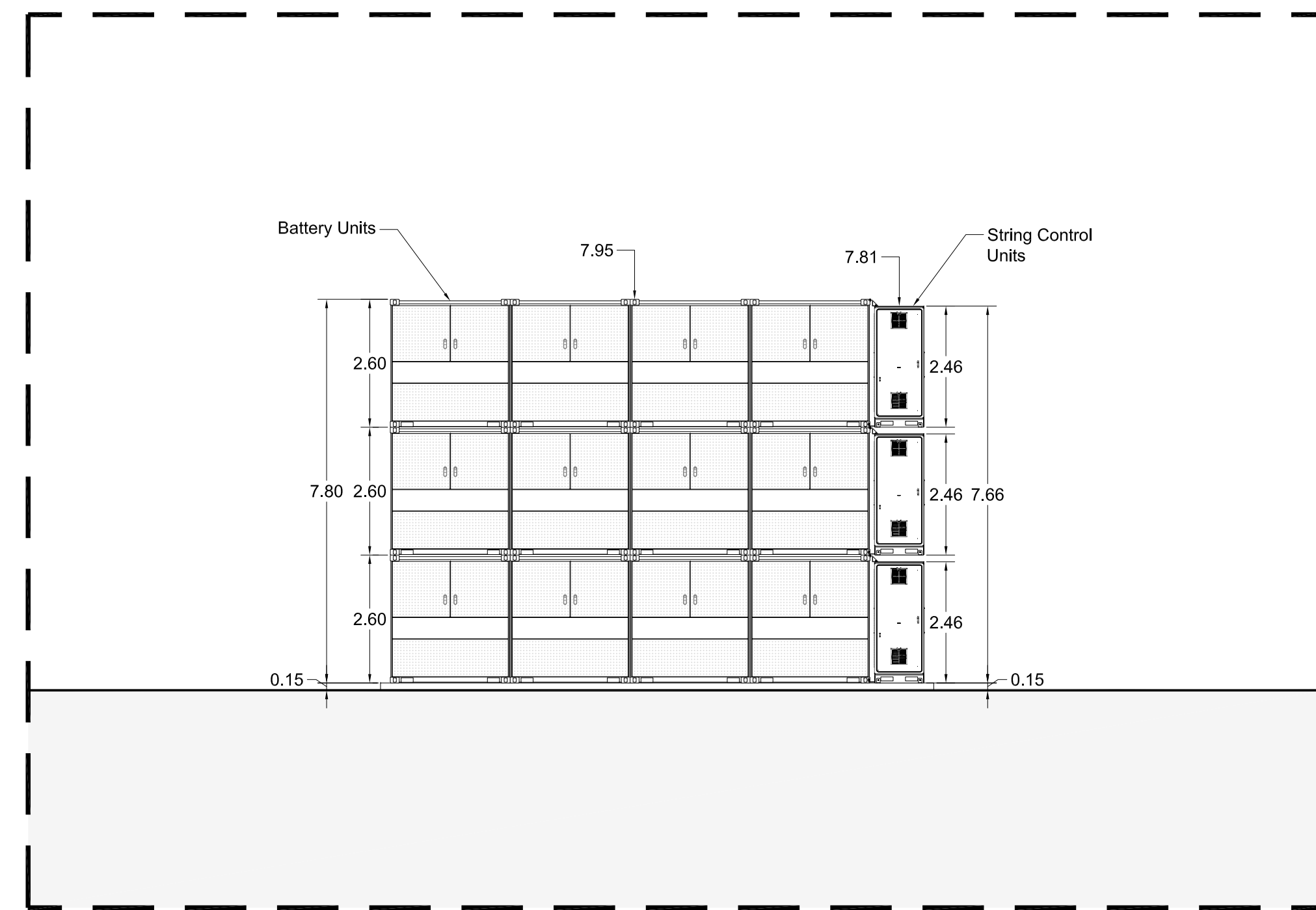
3 TRIPLE STACKED STRING DETAIL Scale: 1:100@A0
